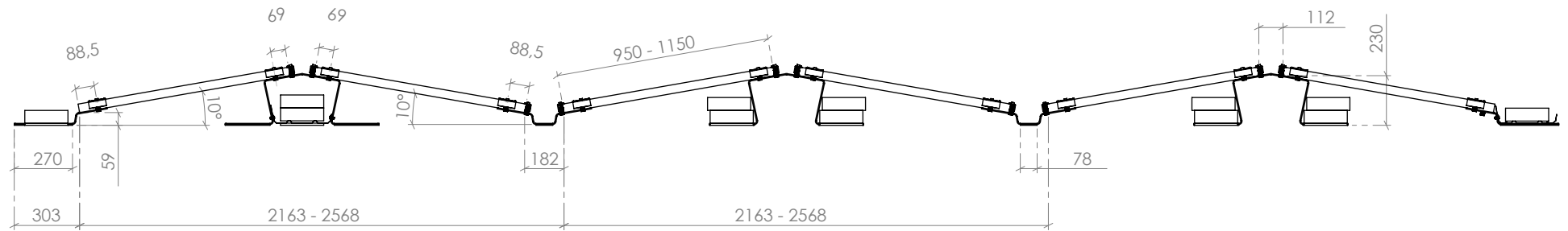
Flat roof S 10+ – 297 mm
