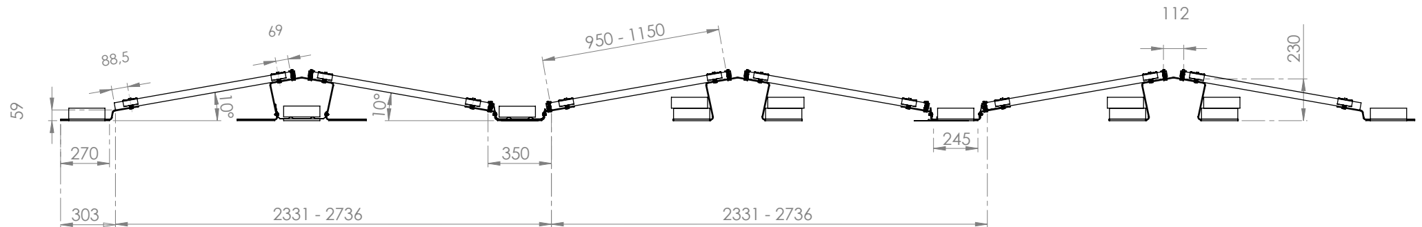
Flat roof S 10+ – 464 mm
